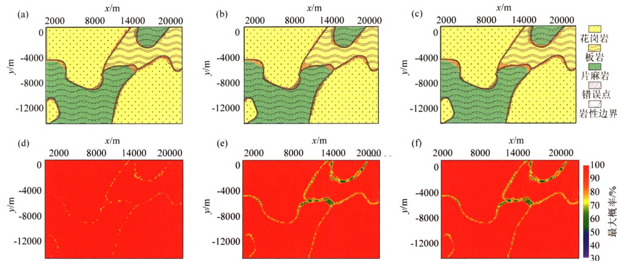
a~f 分别表示对于 250 个训练样本点的传统高斯分类、固定带宽的核密度估计、自适应带宽的核密度估计的贝叶斯分类结果以及其对应的概率分布 Figures a~f respectively represent the Bayesian classification results, corresponding probability distribution map of the traditional Gaussian classification, fixed bandwidth kernel density estimation, adaptive bandwidth kernel density estimation for 250 training sample points
