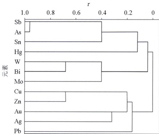
图 3 亮甲峪测区土壤地球化学 R 型聚类谱系 Fig.3 The R-type clustering of soil geochemistry of the Liangjiayu district
