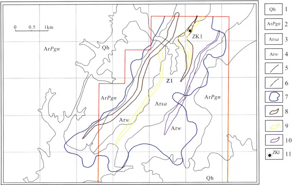
1—第四系冲洪积亚黏土、亚砂土;2—潘庄组变质二长花岗岩;3—三门店组黑云斜长变粒岩夹斜长角闪岩;4—湾杖子组斜长角闪岩夹角闪斜长变粒岩;5—实测地质界线;6—推测地质界线;7—综合异常范围;8—W、Mo、Bi 异常带;9—Au、Cu、Pb、As、W 异常带;10—As、Sb、Hg、Cu、Pb 异常带;11—钻孔位置及编号 1—alluvial clay, sub-sand of Quaternary;2—metamorphic adamellite of Panzhuang formation;3—biotite plagioclase granulite of Sanmendian formation;4—amphibolite and granulite of Wanzhangzi formation;5—measured geological boundary;6—inference geologic boundary;7—synthetic anomaly belt;8—W, Mo, Bi anomaly belt;9—Au, Cu, Pb, As, W anomaly belt;10—As,Sb,Hg,Cu,Pb anomaly belt;11—the location and number of borehole
