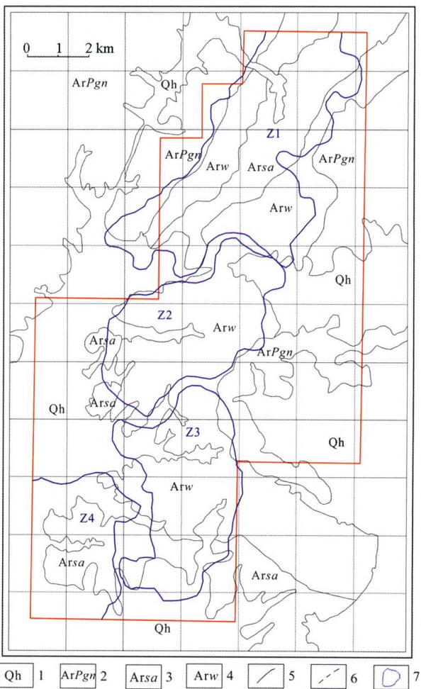
图 4 亮甲峪测区综合异常分布 Fig.4 The comprehensive anomaly distribution of the Liangjiayu area 1—第四系冲洪积亚黏土、亚砂土;2—潘庄组变质二长花岗岩;3—三门店组黑云斜长变粒岩夹斜长角闪岩;4—湾杖子组斜长角闪岩夹角闪斜长变粒岩;5—实测地质界线;6—推测地质界线;7—综合异常范围 1—alluvial clay, sub-sand of Quaternary;2—metamorphic adamellite of Panzhuang formation;3—biotite plagioclase granulite of Sanmendian formation;4—amphibolite and granulite of Wanzhangzi formation;5—measured geological boundary;6—inference geologic boundary;7—synthetic anomaly range
