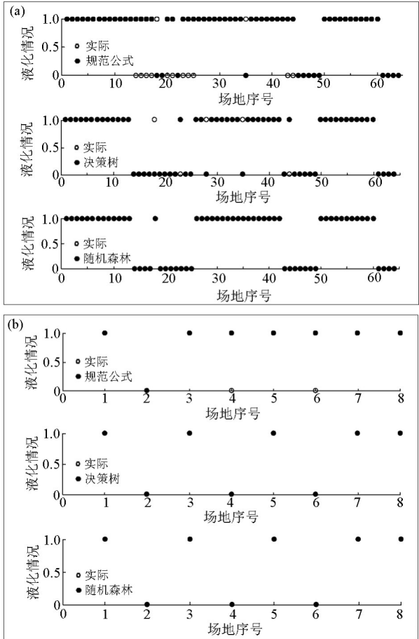
图 5 模型训练(a)及预测结果(b) Fig.5 Training results(a) and test results(b) 万方数据 of prediction model
