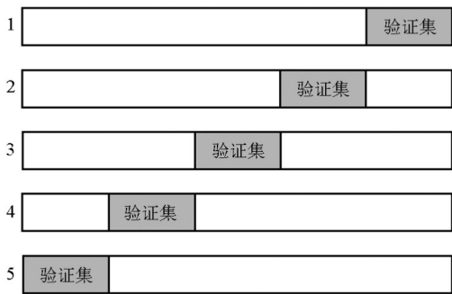
图 4 交叉验证示意 Fig.4 Cross-validation sketch
