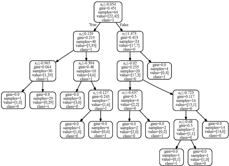
图 3 决策树分类过程示意 Fig.3 Decision tree classification process
