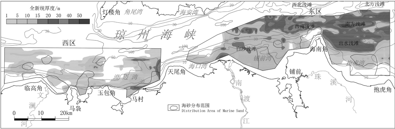
图6 研究区全新统沉积厚度图 Fig.6 The Holocene sediment thickness in the study area
