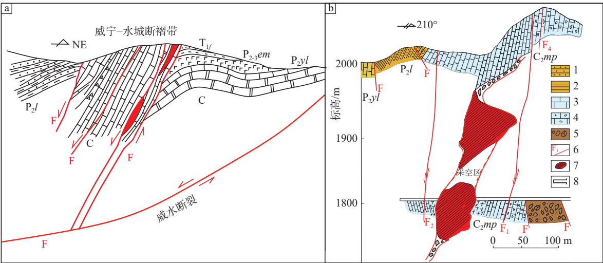
图 15 青山铅锌矿床矿化样式图(a, 据韩润生等, 2020 修改; b, 据钱建平, 2001 修改) a: T_{1f} —下三叠统飞仙关组; P_{2,3em} —峨眉山玄武岩; P_{2yl} —中二叠统阳新组一阶; P_2l —中二叠统梁山组; C—石炭系; b: 1—碎屑岩; 2—页岩; 3—灰岩; 4—角砾状灰岩; 5—角砾岩; 6—断裂; 7—矿体; 8—坑道 Fig.15 Mineralization pattern of the Qingshan lead-zinc deposit(a, modified from Han Runsheng et al., 2020; b, modified from Qian Jianping, 2001) a: T_{1f} —Lower Triassic Feixianguan Formation; P_{2,3em} —Emeishan basalts; P_{2yl} —The first stage of Middle Permian Yangxin Formation; P_2l —Middle Permian Liangshan Formation; C—Carboniferous; b: 1—Clastic rock; 2—Shale; 3—Limestone; 4—Brecciated limestone; 5—Breccia; 6—Fault; 7—Ore body; 8—Tunnel
