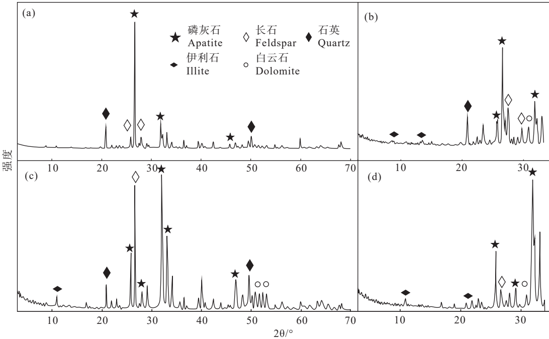
图 7 磷矿石和含磷泥岩 X 射线衍射强度图谱 a—含磷硅质泥岩 (X-JN0); b—含磷硅质泥岩 (X-HP1); c—含磷硅质泥岩 (X-XSC1); d—泥质条带状磷块岩 (X-HP2) Fig.7 X-ray diffraction intensity pattern of phosphate rock and phosphorous mudstone a-Phosphorous siliceous mudstone (X-JN0); b- Phosphorous siliceous mudstone (X-HP1); c-Phosphorous siliceous mudstone (X-XSC1); d- Argillaceous banded phosphorite (X-HP2)
