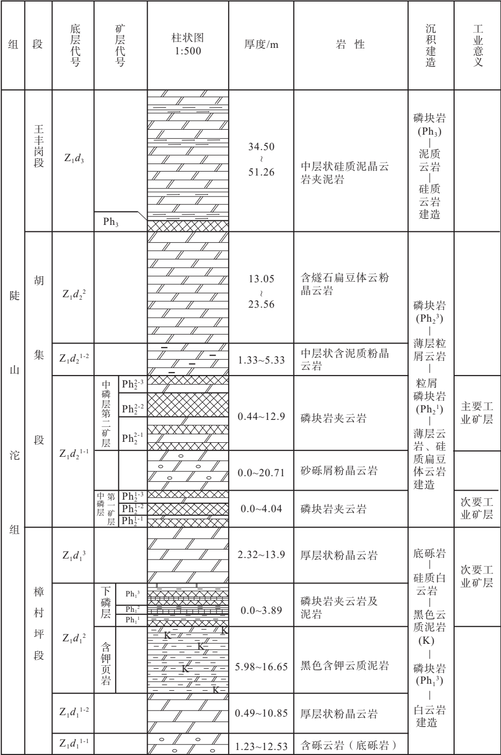
图 2 宜昌磷矿含磷岩系柱状图(据杨刚忠等, 2008 修改) Fig.2 Histogram of phosphate rock series in Yichang phosphate deposit (modified from Yang Gangzhong et al., 2008)
