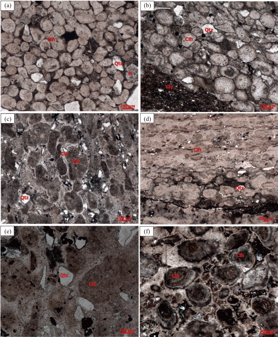
图 5 胶磷矿石显微镜下特征 a—团粒状胶磷矿，凝胶体；b—胶磷矿与泥质条带界线清晰；c—玉髓环绕胶磷矿生长；d—条带状胶磷矿；e—含磷泥岩，砂屑结构；f—泥质胶磷矿，凝胶结构、微晶结构；Clh—胶磷矿；Cly—黏土矿物；Qtz—石英 Fig.5 Microscopic characteristics of collophanite a—Agglomerated phosphate rock, gel; b—Clear boundary between phosphate rock and argillaceous strip; c—Growth of chalcedony surrounding collophanite; d—Banded phosphate rock; e—Phosphorus-bearing mudstone, sand debris structure; f—Argillaceous collophanite, gel structure, microcrystalline structure; Clh—Collophanite; Cly—Clay minerals; Qtz—Quartz
