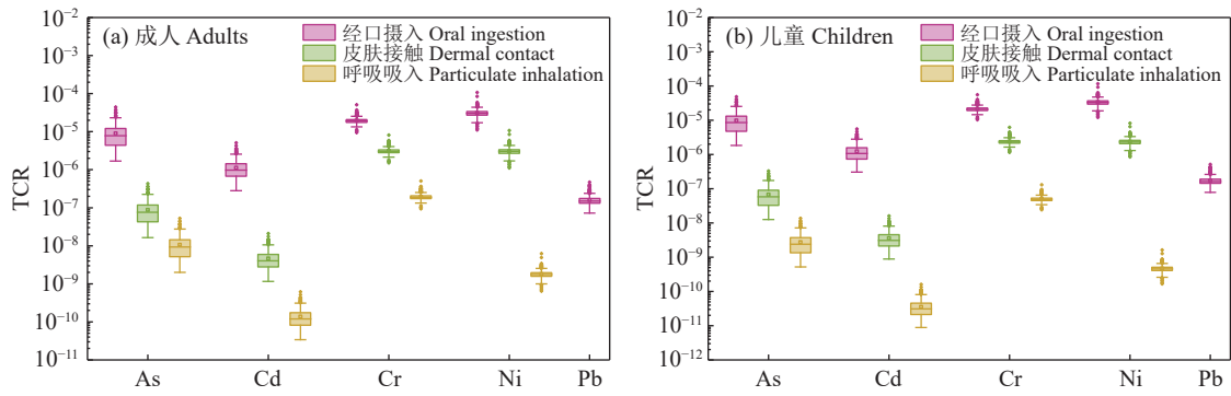
图 6 不同重金属和暴露途径的致癌风险指数 Fig.6 Carcinogenic risk index of different heavy metals and exposure routes
