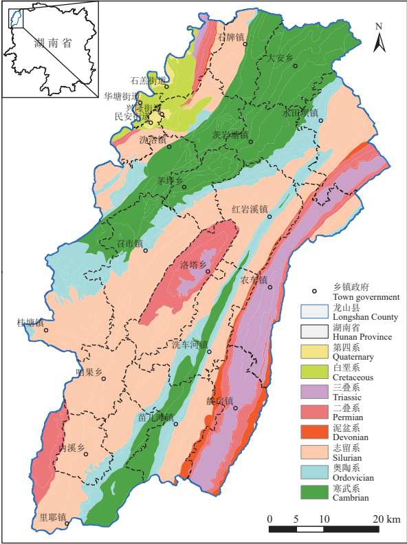
图 1 区域地质简图及龙山县位置(李晨阳等, 2019) Fig.1 Regional geological map and location of Longshan County(after Li Chenyang et al., 2019)
