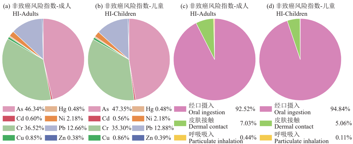
Fig.4 Non-carcinogenic risk index of different heavy metals and exposure routes
