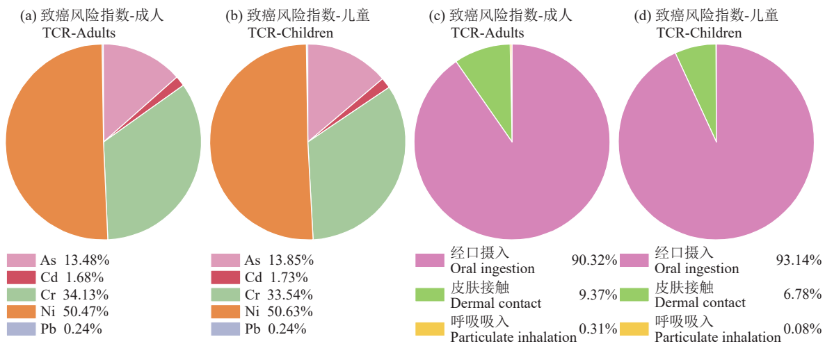
图 7 不同重金属和暴露途径对致癌风险指数的平均贡献率 Fig.7 Average contribution rates of different heavy metals and exposure routes to carcinogenic risk index
