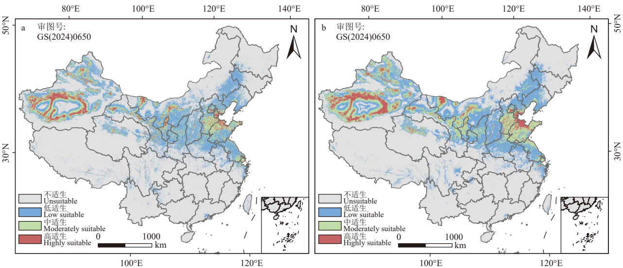
图 3 现代气候模式下有 (a) 和无 (b) 人类活动干扰的柽柳适生区分布 Fig.3 Distribution of T. chinensis suitability zones with (a) and without (b) anthropogenic disturbance under modern climate models
