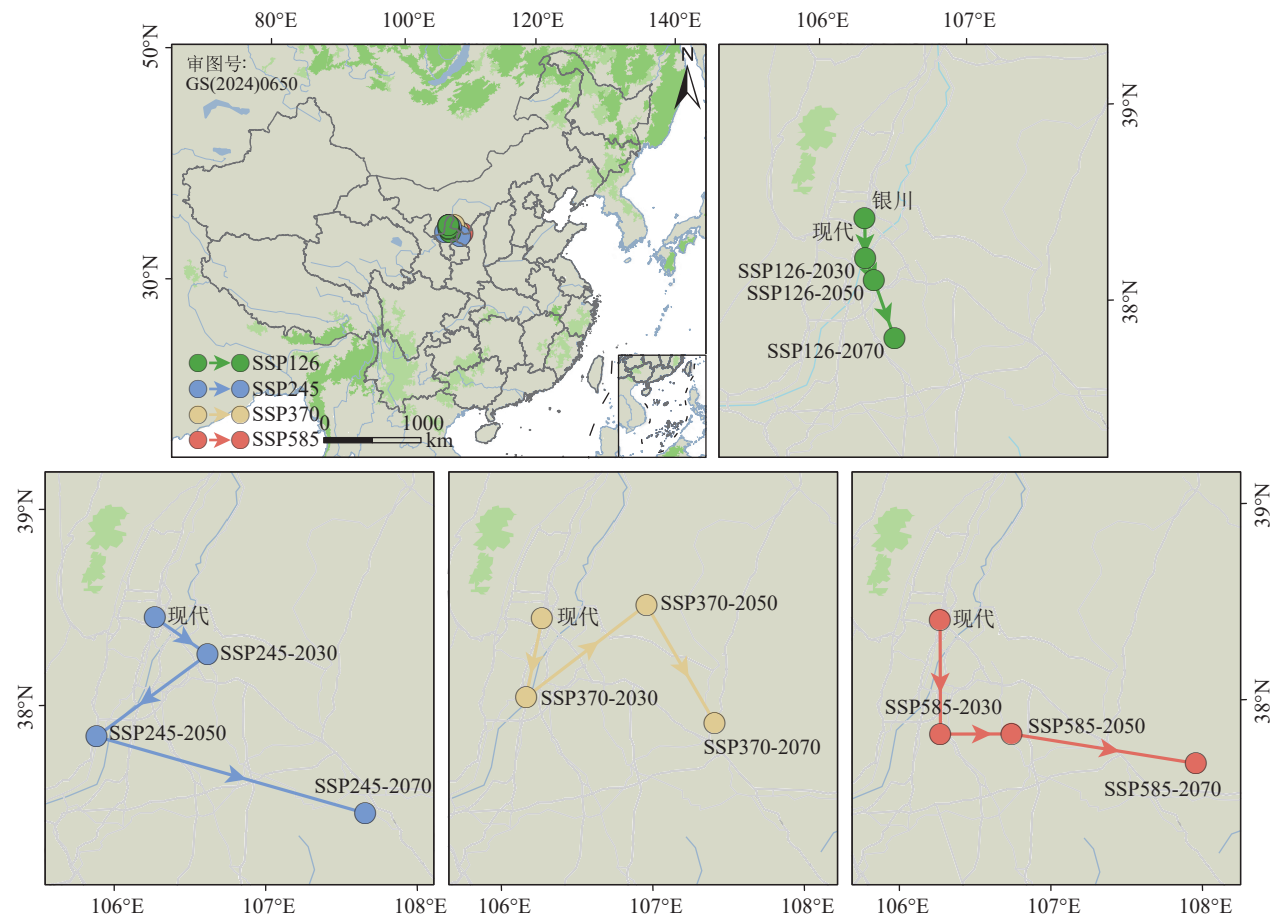
图 7 不同气候情景下怪柳适生区分布中心迁移位置 Fig.7 Location of the center of distribution of tamarisk fitness zone migration under different climate scenarios
