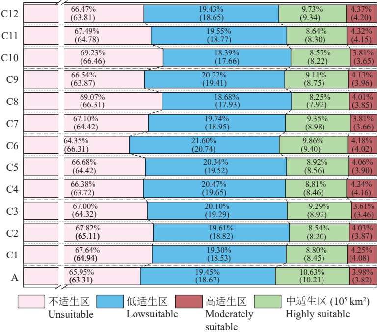
图 5 不同气候变化情景下怪柳的适生区面积及其占比 Fig.5 Area and percentage of T. chinensis 's suitable habitat under different climate change scenarios
