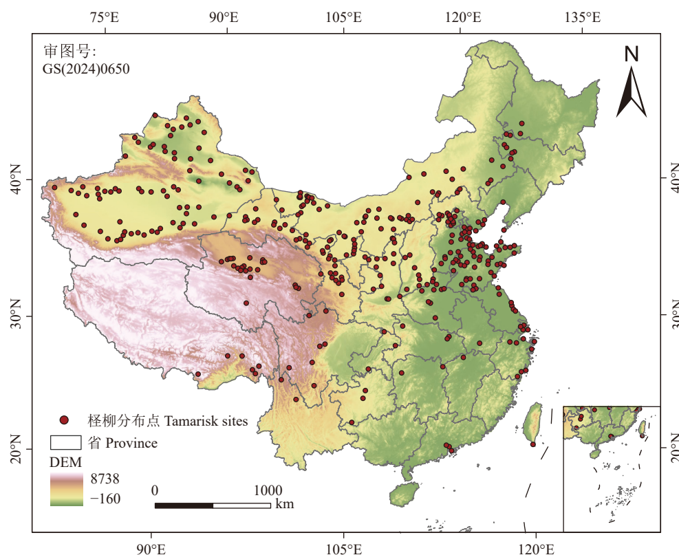
图 1 筛选后的怪柳分布记录 Fig.1 Distribution records of screened T. chinensis
