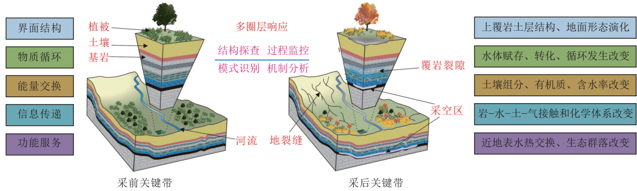
图 2 地球关键带岩-土-水的关联性 Fig.2 Correlation between rock-soil-water in the Earth's critical zone
