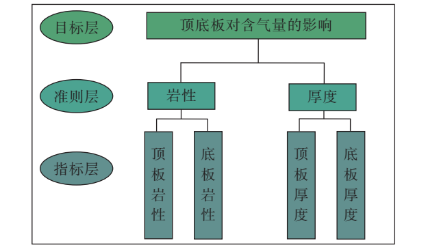
图 12 影响因素评价层次结构 Fig. 12 Hierarchical structure of the evaluation of influencing factors
