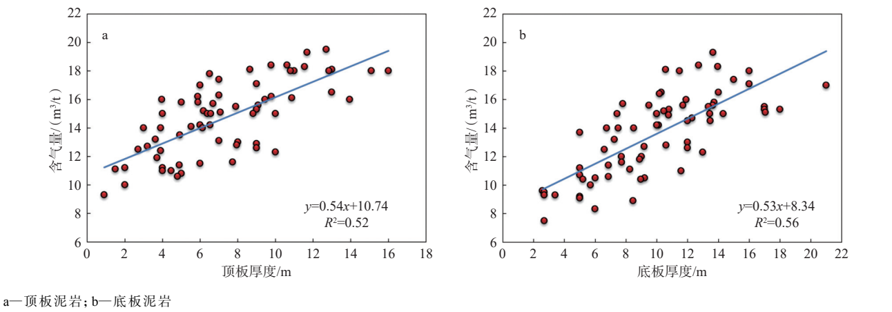
图 11 顶底板泥岩厚度与煤层含气量的关系 Fig. 11 Relationship between hanging- and foot-wall mudstone thickness and coal seam gas content (a) Hanging-wall mudstone; (b) Foot-wall mudstone
