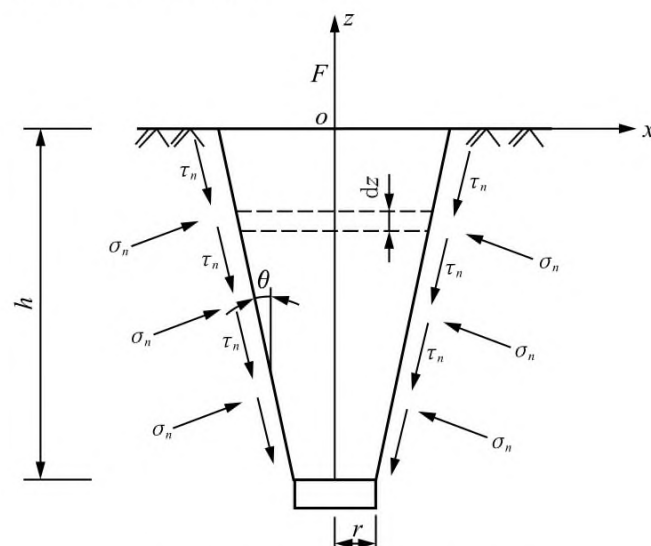
图 2 锚板抗拔的力学模型 Fig.2 Mechanical model for the uplift anchor plates
