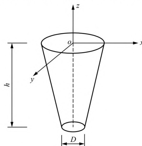
图 1 圆形锚板基础破裂面空间形状 Fig.1 Spatial failure shape of the foundation with circular anchor plates
