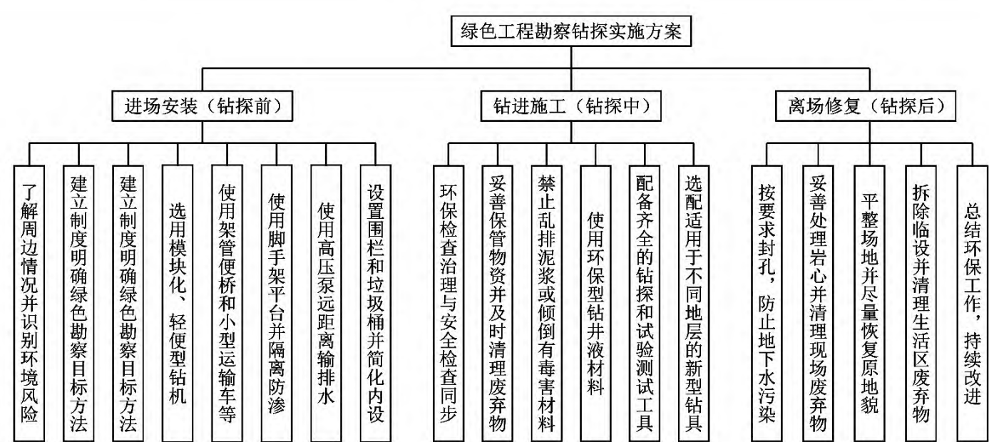
图 1 绿色工程勘察钻探实施方案 Fig.1 Drilling solutions for green engineering investigation
