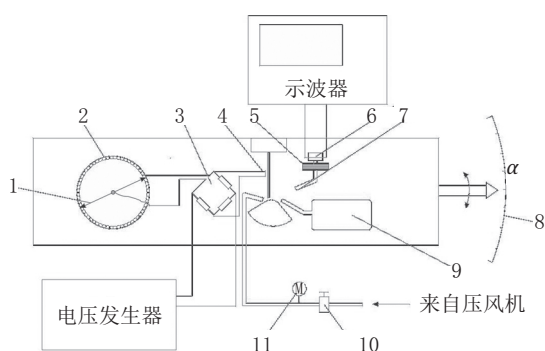
Fig.4 Jet generator
