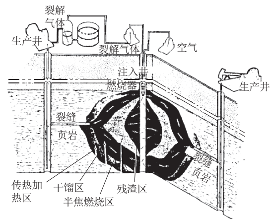
图 1 TIS 技术原理示意 [18] Fig.1 Schematic diagram of TIS
