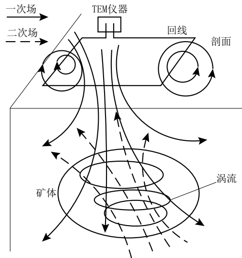
图5 瞬变电磁法原理示意 Fig.5 Schematic diagram of the transient electromagnetic method
