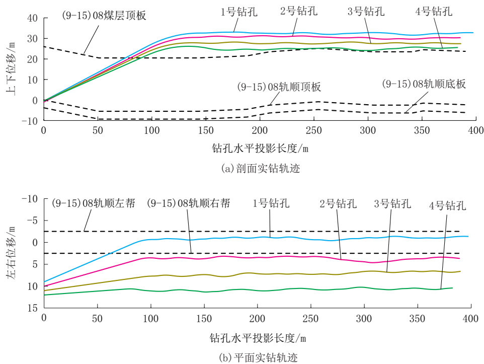
图3 穿层定向长钻孔实钻轨迹 Fig.3 As-drilled trajectories of the cross-bed directional long boreholes
