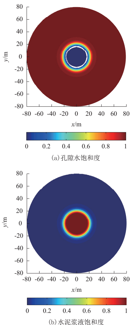
图2 各向同性地层注浆孔周围孔隙水和水泥浆液饱和度分布 Fig.2 Saturation distribution of pore water and cement grouting around the borehole in the isotropic formation
