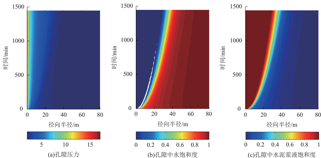
图 3 注浆过程中孔隙压力和饱和度随注浆时间的变化规律(表 1 中第 1 行案例) Fig.3 Change law of pore pressure and pore water saturation with time in the process of cement grouting
