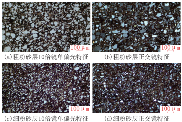
图 1 6-2 号岩样电镜测试结果 Fig.1 Electron microscopy test results of rock sample No.6-2
