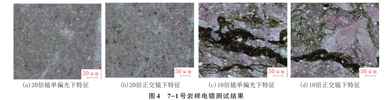
Fig.4 Electron microscopy test results of rock sample No.7-1
