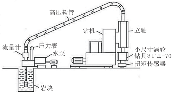
图5 试验研究 3ГД-70 型钻具工作性能的试验台 Fig.5 Stend for experimental research on working performance of turbo drill 3ГД-70
