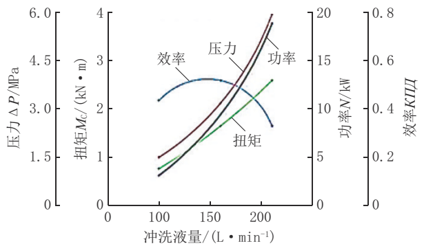
图4 转速 n=500 r/min 时 3ГД-70 型涡轮钻具性能参数与冲洗液流量的关系曲线 Fig.4 Dependence of the turbo drill 3ГД-70 performance parameters from drilling fluid quantity while n=500 r/min
