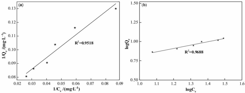
图 8 高岭石吸附氟离子的(a) Langmuir、(b) Freundlich 吸附等温线 Fig. 8 (a) Langmuir and (b) Freundlich adsorption isotherms of fluoride ions on kaolinite
