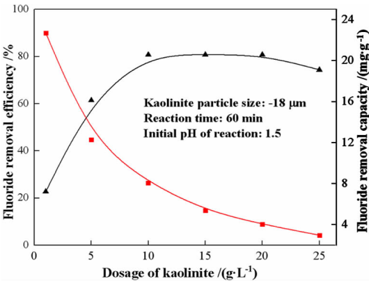
图 4 高岭石用量对氟离子去除率的影响 Fig. 4 Effect of kaolinite dosage on fluoride removal efficiency
