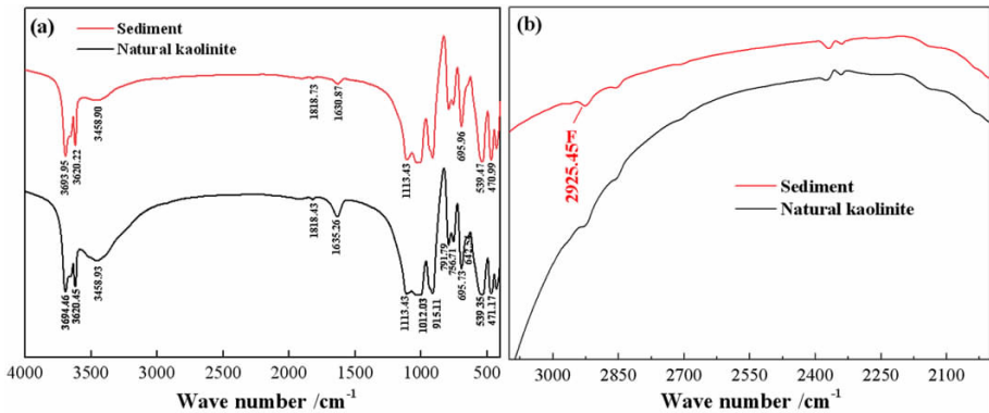
图 9 天然高岭石及除氟渣的 FTIR 全谱(a), FTIR 局部窄谱(b) Fig. 9 (a) FTIR full spectrum and (b) FTIR local narrow spectrum of natural kaolinite and defluorinated residue
