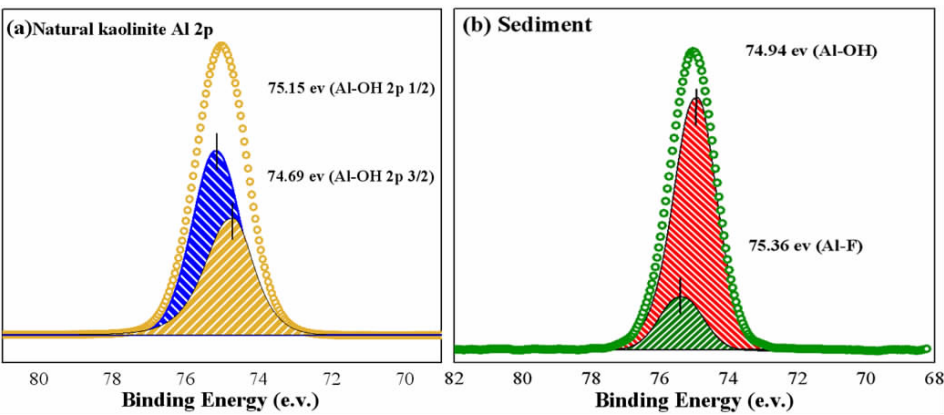
图 11 Al 2p XPS 图谱:(a)天然高岭石 Al 2p3/2, Al 2p1/2;(b)氟离子吸附后高岭石的 Al 2p Fig. 11 XPS Atlas of Al 2p: (a) Al 2p 3/2 of natural kaolinite and Al 2p 1/2; (b) Al 2p of kaolinite adsorbed by fluoride ions
