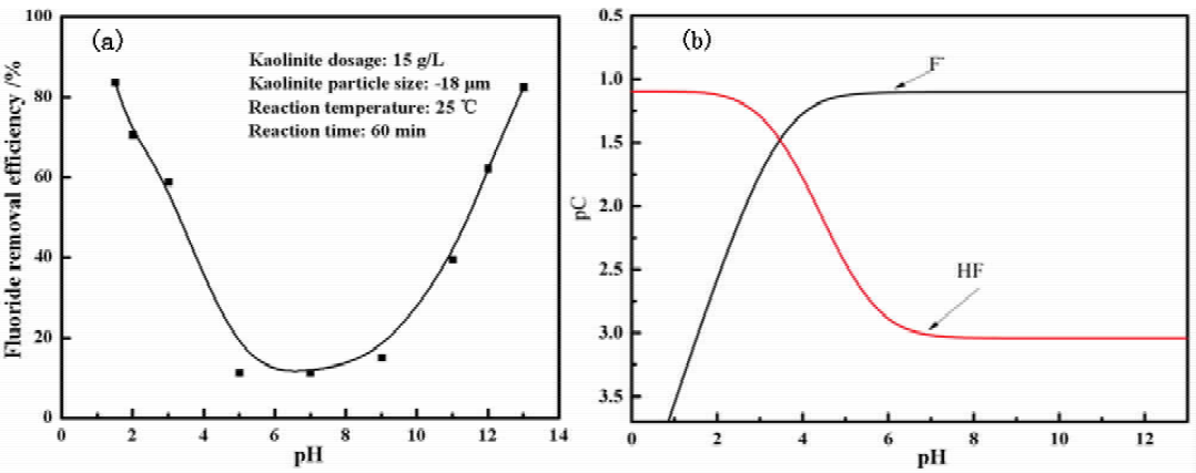
图 3 (a) 溶液 pH 值对氟离子去除率的影响; (b) 模拟含氟废液的 pC - pH 图 Fig. 3 (a) Effect of solution pH on removal efficiency of fluoride ions; (b) Simulated pC - pH diagram of fluoride - containing wastewater
