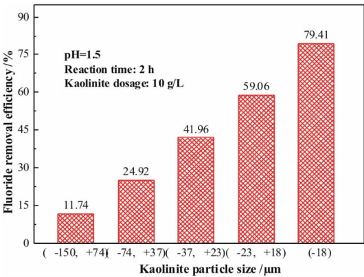
图 5 高岭石粒度对氟离子去除率的影响 Fig. 5 Effect of Kaolinite Particle Size on Fluoride Removal Efficiency
