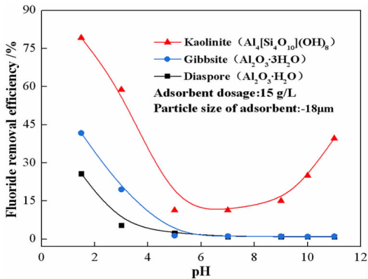
图 1 pH 值对三种铝硅酸盐矿物除氟的影响 Fig. 1 Effect of pH on defluorination of three aluminosilicate minerals
