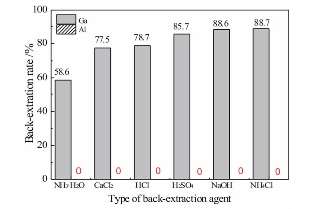
图10 反萃取剂种类对镓、铝反萃取率的影响 Fig. 10 Effect of back-extraction agents on back-extraction rate of Ga and Al
