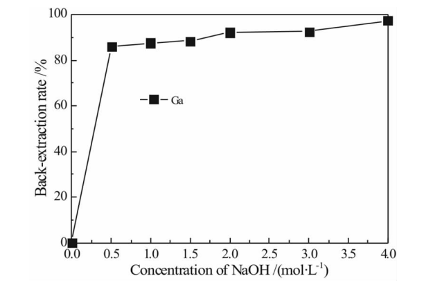
图11 氢氧化钠浓度对镓反萃取率的影响 Fig. 11 Effect of concentration of NaOH on back-extraction rate of Ga
