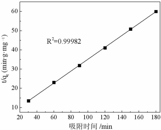
图 9 CSCC 吸附 \text{SO}_4^{2-} 准二级动力学拟合图 Fig. 9 The second order dynamic fitting diagram of \text{SO}_4^{2-} adsorbed by coconut shell activated carbon
