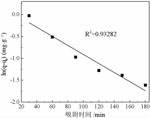
图 8 CSCC 吸附 \text{SO}_4^{2-} 准一级动力学拟合图 Fig. 8 The first order dynamic fitting diagram of \text{SO}_4^{2-} adsorbed by coconut shell activated carbon
