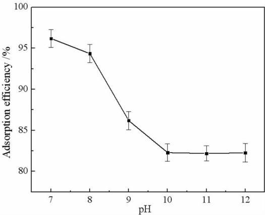
图6 pH 对吸附效率的影响 Fig. 6 Effects of pH on adsorption efficiency
