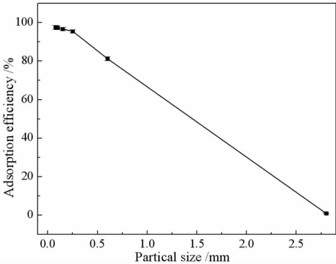
图 2 粒径大小对吸附效率的影响 Fig. 2 Effects of particle size on adsorption efficiency
