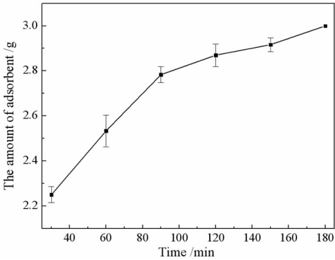
图 7 活性炭吸附量和吸附时间的关系 Fig. 7 Relationship between adsorption amount and adsorption time
