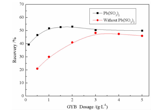
图2 GYB 药剂用量对黑钨矿浮选的影响 Fig. 2 The results of GYB dosage test of wolframite flotation
