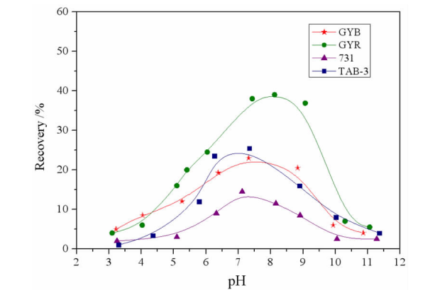
图 1 pH 对黑钨矿浮选回收率的影响 Fig. 1 Relationship of pH and collecting capability on wolframite
