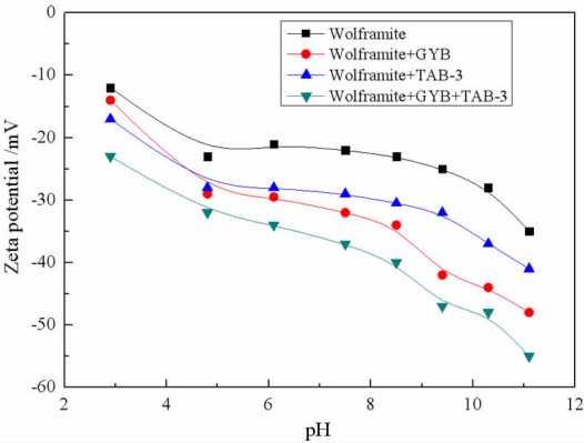
图 7 黑钨矿表面 Zeta 电位与 pH 的关系 Fig. 7 Relationship between pH and Zeta potential of wolframite with different collectors
