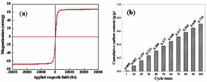
图 9 低品质多金属矿矿相重构磨选产品的性能表征:(a)磁性能,(b)CO 2 分解性能 Fig. 9 Performance characterization of the separated products from the low - grade of manganese ore via mineral phase reconstruction, grinding and separation process
