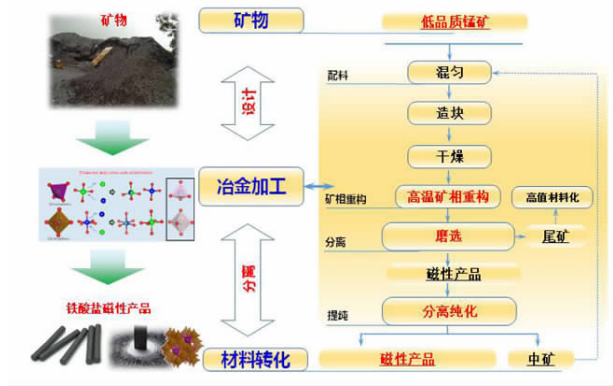
图3 低品质多金属矿资源矿相重构-分选原则流程图 Fig. 3 Principle flowsheet of mineral phase reconstruction, grinding and separation process for the low-grade of polymetallic ore resources
