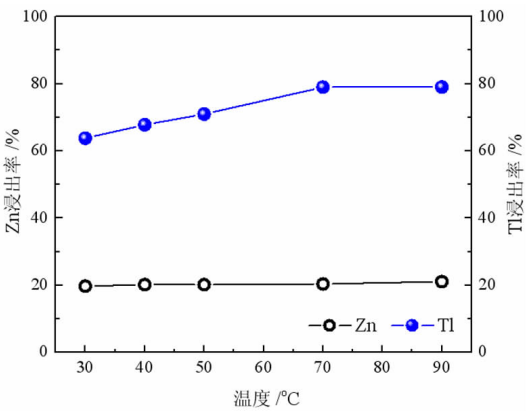
图 3 水浸温度对锌和铊浸出率的影响 Fig. 3 Effect of water leaching temperature on leaching rate of Zn and Tl
