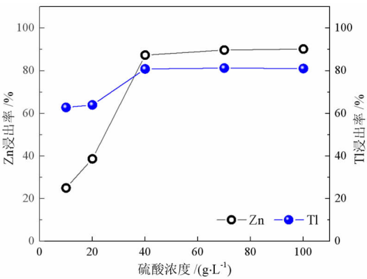
图 4 硫酸浓度对锌和铊浸出率的影响 Fig. 4 Effect of \text{H}_2\text{SO}_4 concentration on leaching rate of Zn and Tl
