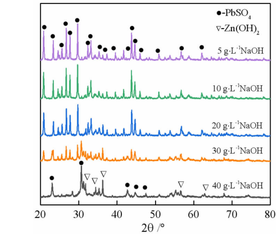
图 8 不同 NaOH 浓度下浸出渣的 XRD 谱 Fig. 8 XRD patterns of the leaching residue at different NaOH concentration
