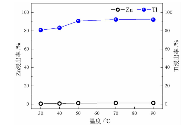
图 10 NaOH 浸出时温度对锌和铊浸出率的影响 Fig. 10 Effect of NaOH leaching temperature on leaching rate of Zn and Tl
