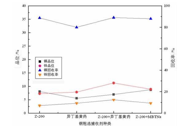
图6 铜粗选捕收剂种类试验结果 Fig. 6 Results of copper roughing collector types tests
