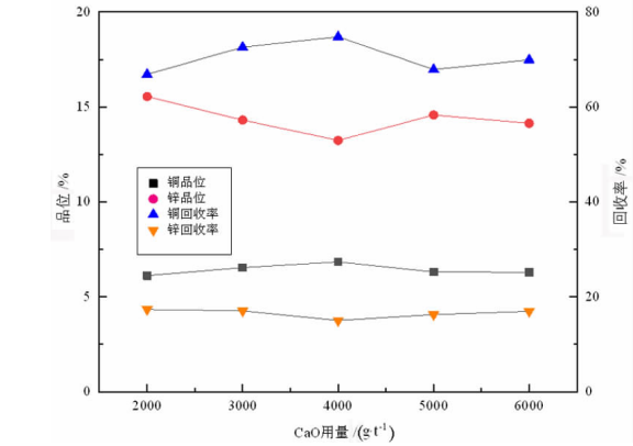
图9 CuSO 4 用量试验结果 Fig. 9 Results of CuSO 4 dosage tests
