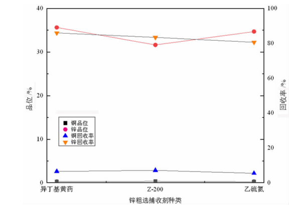
图10 锌粗选捕收剂种类试验 Fig. 10 Results of zinc roughing collector types tests
