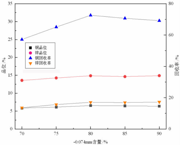
图 3 磨矿细度试验结果 Fig. 3 Results of grinding fineness tests
