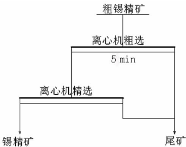
图 6 锡粗精矿精选流程 Fig. 6 Cleaning flowsheet of tin rough concentrate
