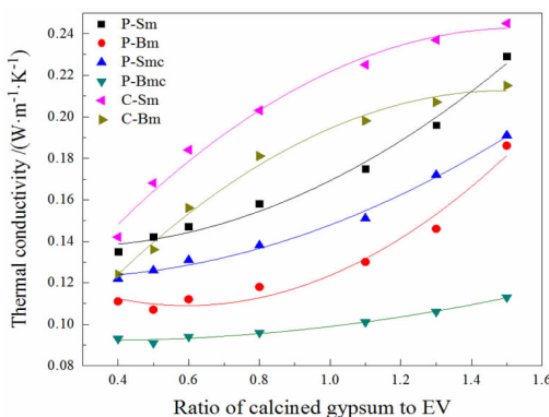
图2 膨胀蛭石保温板的导热系数与烧石膏/膨胀蛭石的关系 Fig. 2 Relationship between thermal conductivity of expanded vermiculite insulation board and calcined gypsum/expanded vermiculite
