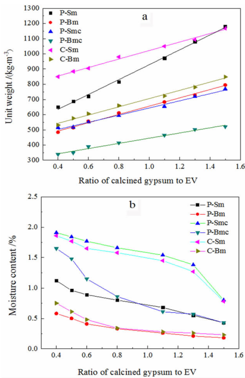
图1 蛭石保温板的密度(a)和含水率(b)与烧石膏/膨胀蛭石质量比的关系 Fig. 1 The relationship between density (a), moisture content (b) of vermiculite insulation board and mass ratio of calcined gypsum/expanded vermiculite
