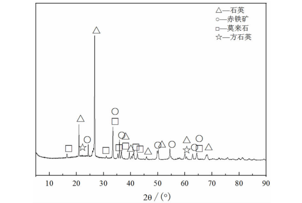
图4 清水泥成品的XRD图谱 Fig. 4 The XRD patterns of the sintering product of Qingshui Zisha clay
