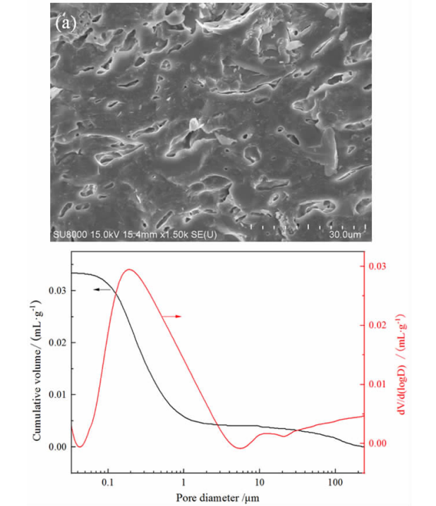
图5 清水泥烧成品的SEM图像(a)和孔径分布图(b) Fig. 5 The SEM image (a) and the pore size distribution (b) of the sintering product of Qingshui Zisha clay
