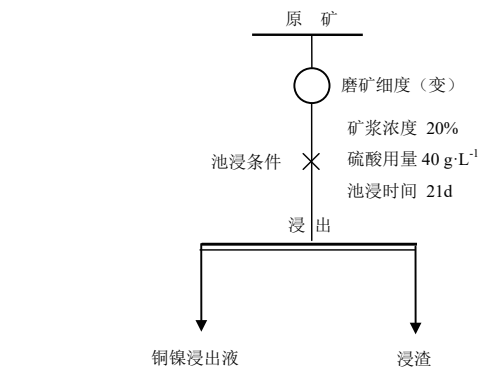
图 3 磨矿细度试验工艺流程及条件 Fig. 3 Process flow and conditions of grinding fineness test
