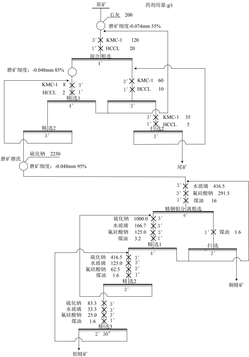
图 7 全流程小型闭路试验流程 Fig. 7 Flow chart of whole process of small closed-circuit of tests
