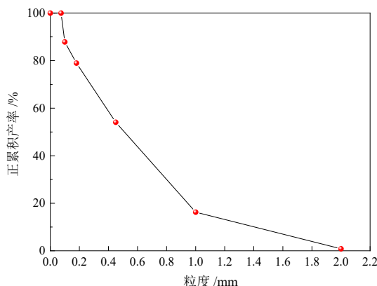
图2 原料的粒度特性曲线 Fig. 2 Particle size characteristic curves of raw materials
