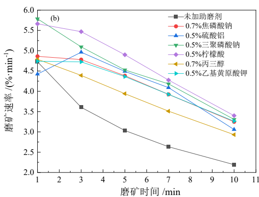
Fig. 8 Effects of grinding aids on grinding rate of -1+0.45 mm and -0.45+0.18 mm particle size
