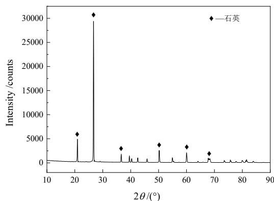
图1 石英X射线衍射图谱 Fig. 1 The X-ray spectra of quartz
