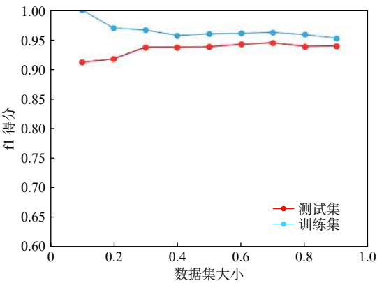
图 3 逻辑回归模型学习曲线和 ROC 曲线 Fig. 3 Learning curve and ROC curve of the logistic regression model
