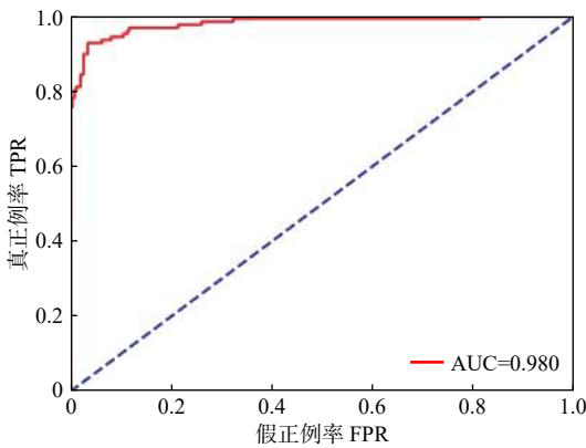
图 3 逻辑回归模型学习曲线和 ROC 曲线 Fig. 3 Learning curve and ROC curve of the logistic regression model
