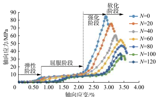
图 8 冻融花岗岩单轴压缩全过程应力-应变曲线 Fig. 8 Uniaxial compressive stress-strain curve of freezing-thawing granite
