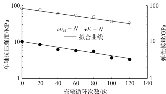
图 9 单轴抗压强度和弹性模量与冻融循环次数的关系 Fig. 9 Uniaxial compressive strength and elasticity modulus as a function of number of freezing-thawing cycles
