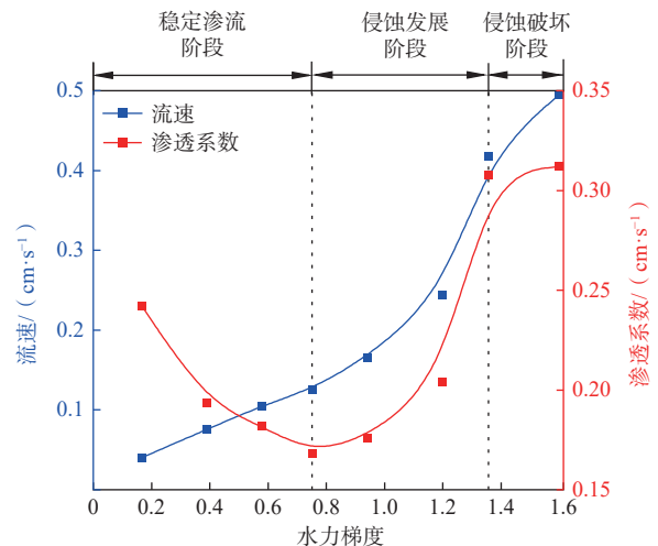
图 4 渗透系数、流速与水力梯度的关系 Fig. 4 Relationship between permeability coefficient, flow velocity, and hydraulic gradient
