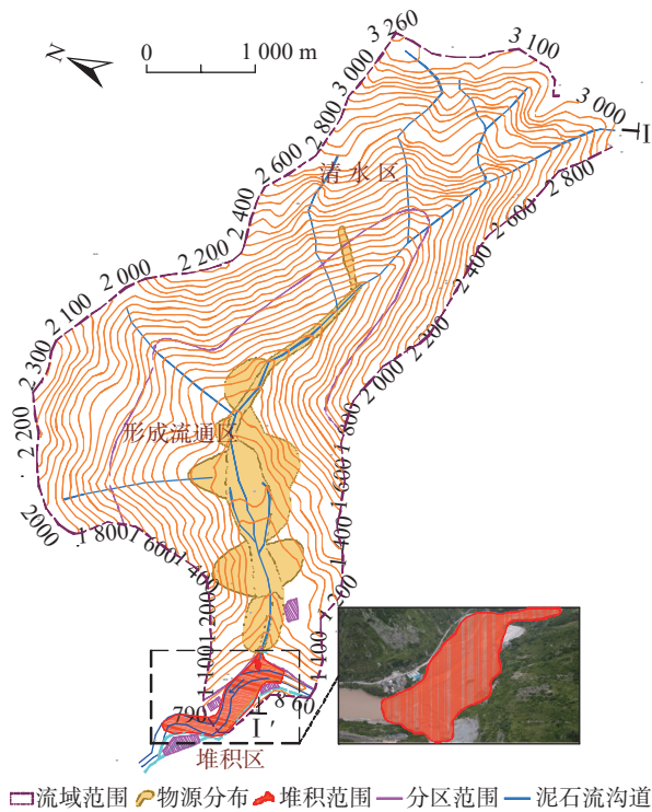
图 1 黑西洛沟泥石流流域及物源分布 Fig. 1 Catchment features and distribution of source materials in Heixiluo gully
