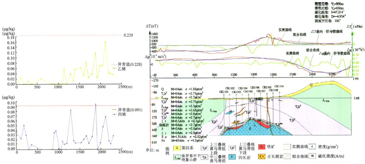
图 4 白象山矿区 11 线物化探综合异常剖面图 Fig. 4 Geophysical and geochemical anomaly profiles of exploration line 11 in the Baixiangshan mine district
