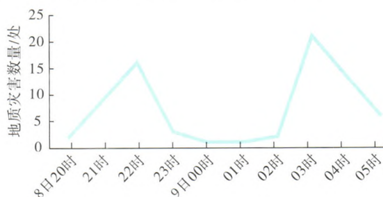
图 5 泰顺县苏迪罗登陆前后各时段地质灾害发生数量 Fig. 5 Amount variation of geological hazards before and after Soudelor landing in Taishun County
