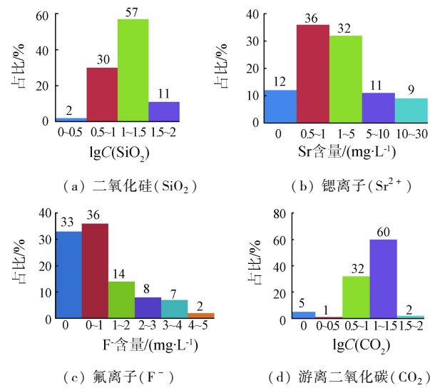
图 6 地热流体微量元素及气体成分分布频率图 Fig. 6 Distribution frequency of trace elements and gas components in geothermal fluids
