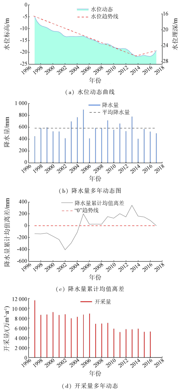
图 5 大王镇南陈官村浅层地下水多年水位动态曲线 Fig. 5 Multi-year dynamic curve of shallow groundwater level in Nanchenguan Village of Dawang Town 万方数据
