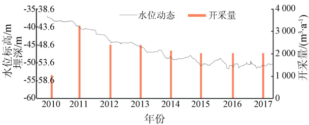
图 6 广饶县大码头乡东燕村深层地下水多年水位动态 Fig. 6 Multi-year dynamic curve of deep groundwater level in Dongyan Village of Damatou Town in Guangrao County
