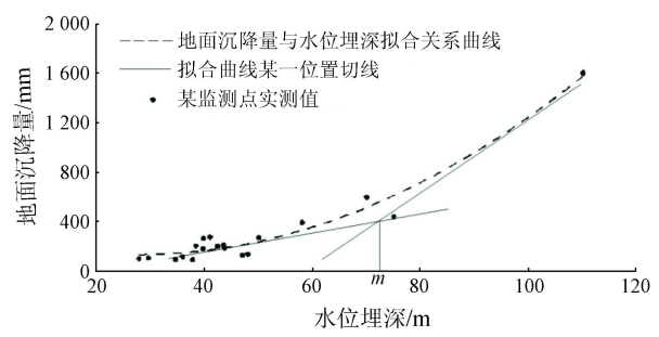
图 12 广饶县地面沉降量与深层地下水位关系 Fig. 12 The correlation curve between land subsidence and deep groundwater level in Guangrao County
