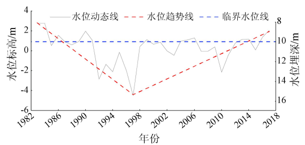
图 11 广饶县甄庙村多年水位动态曲线 Fig. 11 Multi-year dynamic curve of the water level in Zhenmiao Village of Guangrao County
