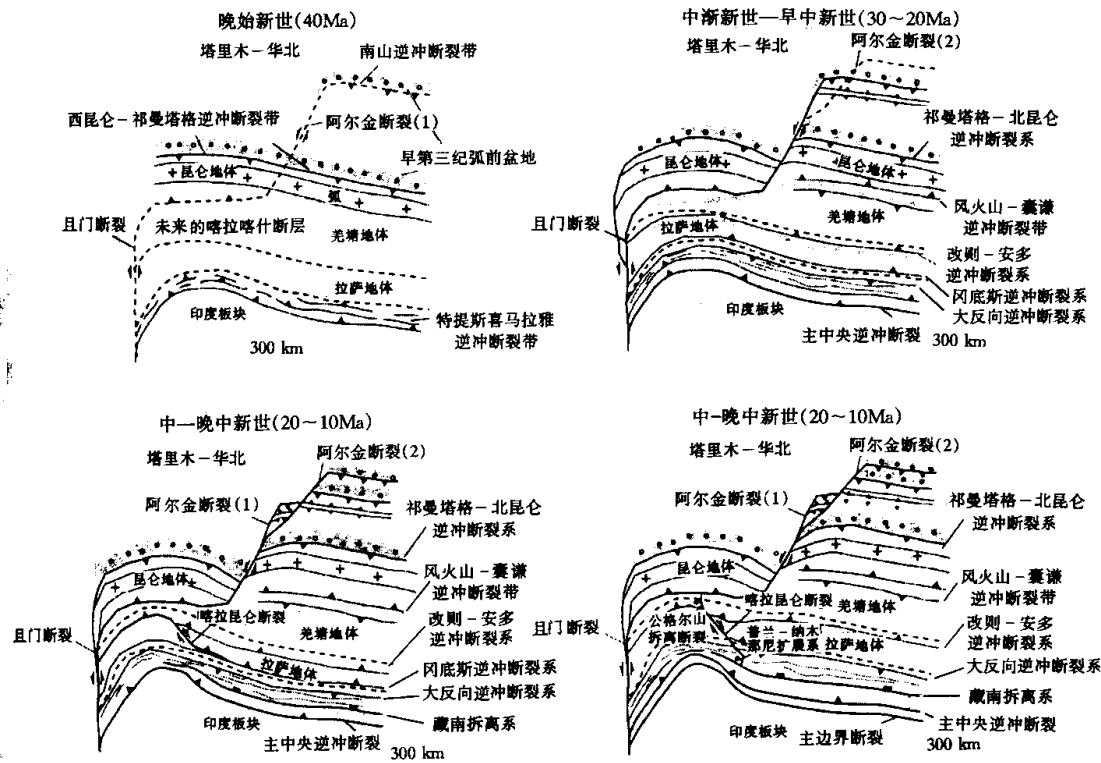
图 5 中喜马拉雅、西北喜马拉雅和青藏高原地区新生代主要构造演化简图 Fig.5 Schematic diagrams showing the evolution of major Cenozoic structures in the central and northwestern Himalaya and the Tibetan plateau regions
