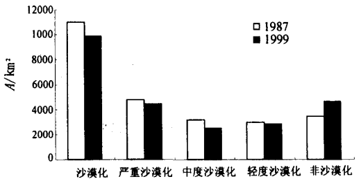
图 2 沙漠化土地面积 Fig.2 Area of desertified land
