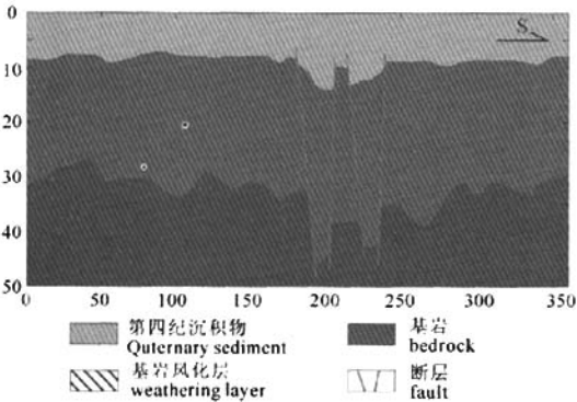
图5 即墨温泉盆地基底断裂地震地质剖面图 (据薛荣俊等, 2005) Fig. 5 Seismic geological section of basement faults in thermal spring basin (from Xue et al., 2005)
