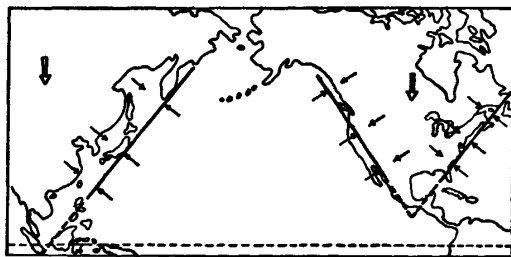
图 4 北美和东亚边缘变形原因的解释 Fig. 4 Interpretation of the causes of deformations on the margins of North America and East Asia
