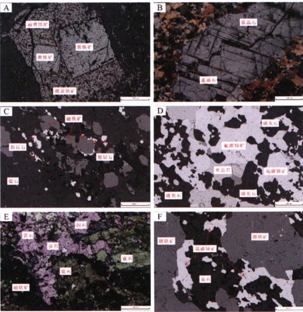
图1 白云鄂博矿石矿物嵌布特征 Fig.1 Dissemination features of Bayan Obo ores
