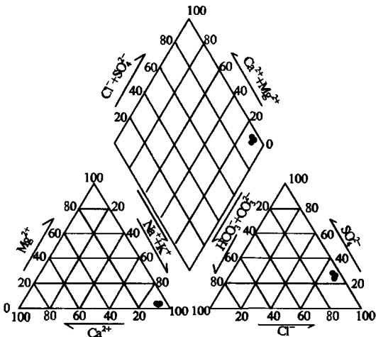
图4 临清地热主要离子的Piper三线图 Fig.4 Main ion piper figure of the Linqing geothermal water
