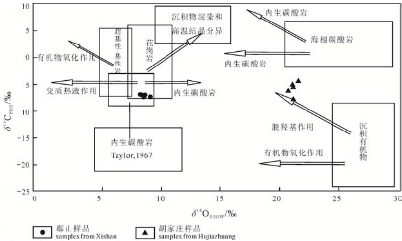
图 5 鲁西郝山、胡家庄稀土矿碳酸盐碳氧同位素分布图(底图据刘家军等, 2004) Fig. 5 Carbon and oxygen isotope distribution of carbonate in Xishan and Hujiashuang rare earth mines in western Shandong (basemap from LIU et al., 2004)
