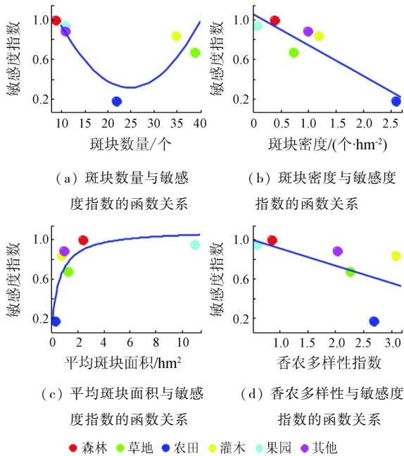
图5 敏感度指数与景观要素破碎指数的函数关系 Fig. 5 Functional relationship between sensitivity index and landscape fragmentation index
