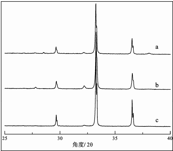
图 2 Ag 3 PO 4 的 XRD 谱图 Fig. 2 XRD patterns of Ag 3 PO 4 a-厦门湾表层海水合成; b-磷空白海水加 KH 2 PO 4 试剂合成; c-Milli-Q 水加 KH 2 PO 4 试剂合成 a-synthesized from Xiamen bay surface seawater; b-synthesized from KH 2 PO 4 reagent in phosphate blank seawater; c-synthesized from KH 2 PO 4 reagent in Milli-Q water
