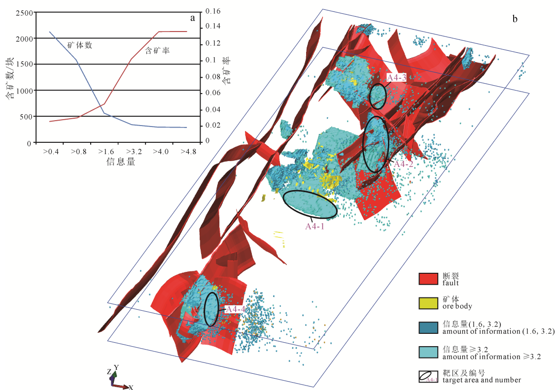
图 6 拉拉铜矿成矿有利区块与靶区划分 Fig. 6 Favorable area for mineralization and division of targets in the Lala mineral deposit
