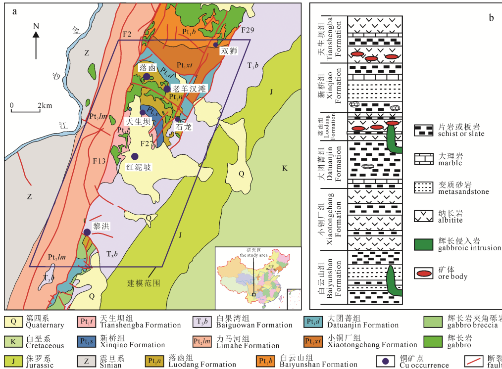
a—矿田地质图; b—河口群地层柱状图。 a—geological map of the orefield; b—stratigraphy of the Hekou Group.
