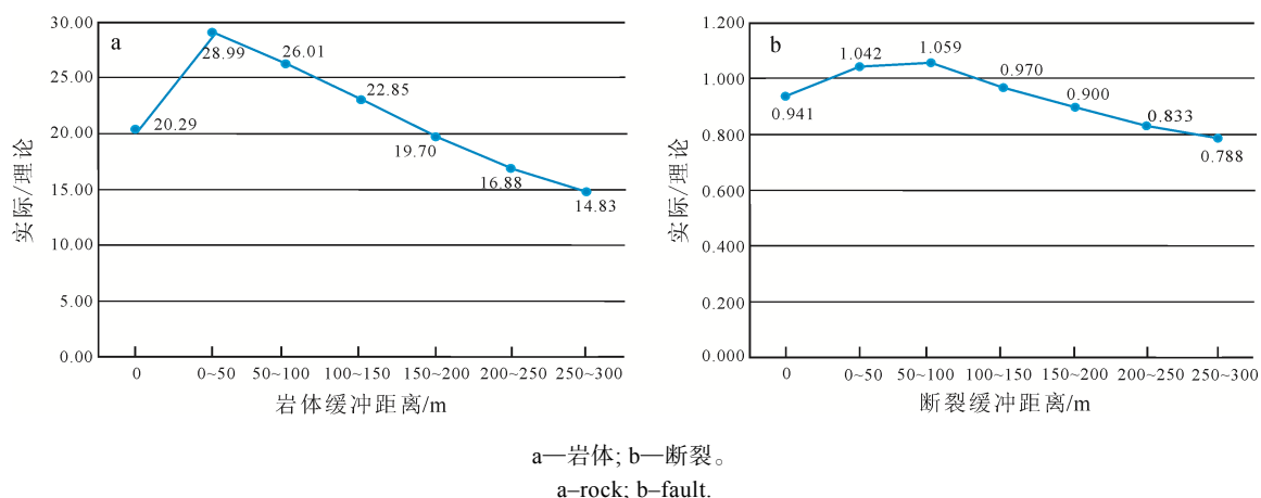
图 5 缓冲区成矿有利信息分析 Fig. 5 Analysis of favorable ore-forming information in buffer zone
