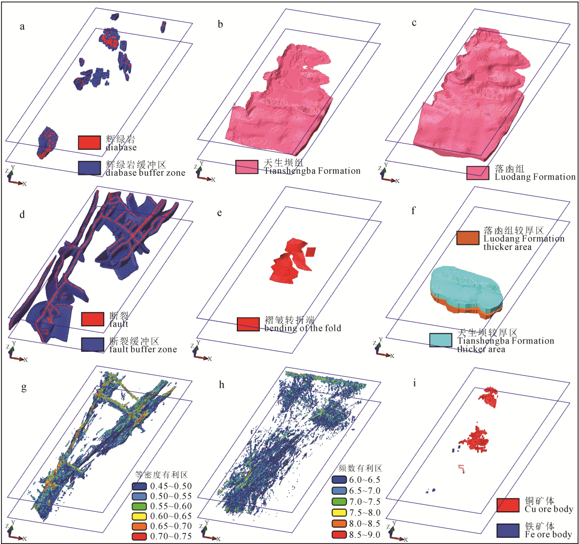
a—辉绿岩及缓冲区; b—天生坝组; c—落凼组; d—断裂及其缓冲区; e—褶皱转折端; f—赋矿地层大于 500 m; g—等密度; h—频数; i—矿体。 a—diabase; b—Tianshengba Formation; c—Luodang Formation; d—fault and buffer; e—hinge zone of fold; f—thickness more than 500 m; g—equidensity; h—fracture frequency; i—orebody.
