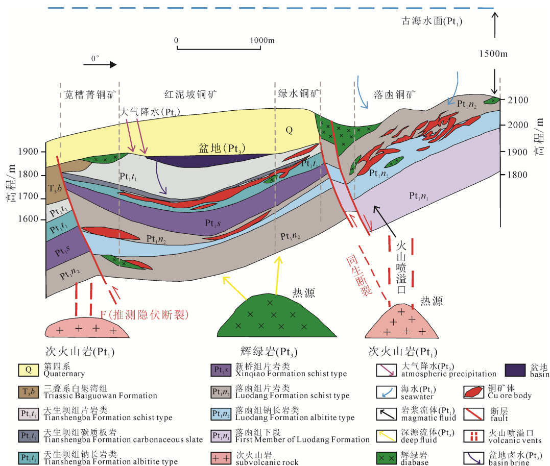
图 2 四川拉拉铜矿成矿模式(据中国地质调查局发展研究中心, 2019 修改) Fig. 2 Metallogenic model of the Lala copper deposit in Sichuan (modified after Development Research Center of China Geological Survey, 2019)
